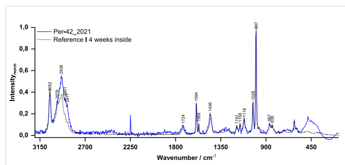
Figure 10: Raman-spectra of ORG applied on the east portal of the Church St. Jacobi in Perleberg. The sample Per-42_2021 was taken in 2021 (blue line). The spectrum was compared to reference material (different batch) that was stored inside for 4 weeks (black dotted line). The spectra were recorded on a WiTec Raman-Microspectrometer using a 532 nm laser. © Fraunhofer ISC
