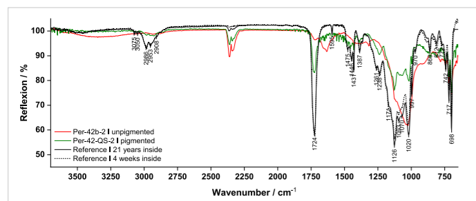
Figure 9: FTIR-spectra of pigmented and unpigmented ORG applied on the east portal (south) of the Church St. Jacobi in Perleberg. The spectra were compared to reference materials (different batches) that were stored inside for either 21 years (black solid line) or 4 weeks (black dotted line). The spectra were recorded with a ThermoFisher Micro-IR-Spectrometer (Nicolet 6700 equipped with a Nicolet continuum FTIR microscope). © Fraunhofer ISC
