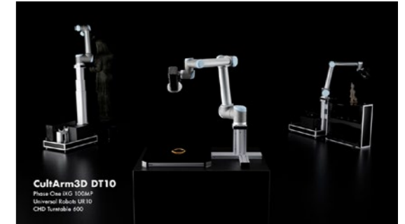
Figure 1: Three variants of the CultArm3D System for different digitization volumes
